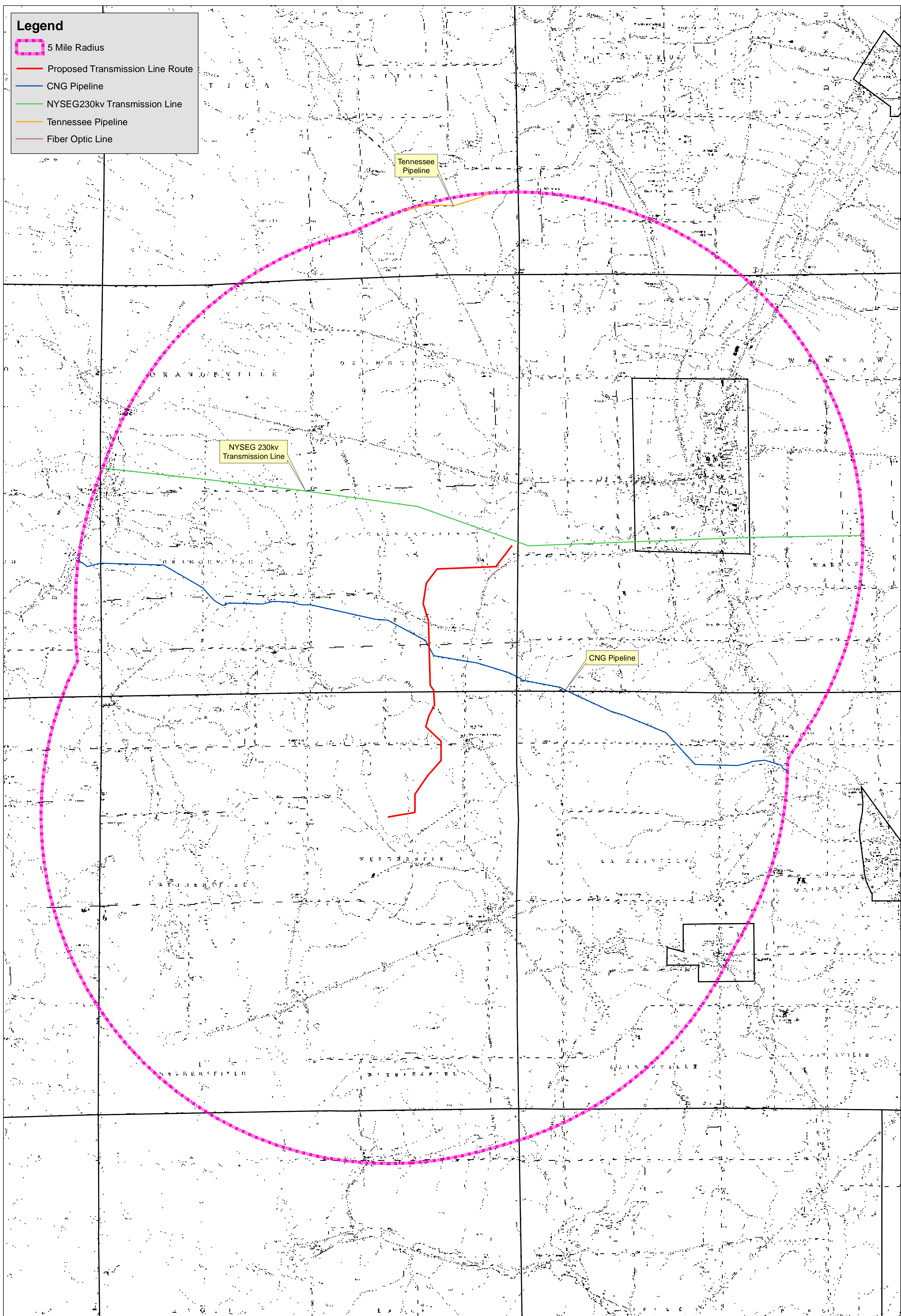
Exhibit 2-1 Relationship to Existing Electric & Gas Facilities Wethersfield-Orangeville Noble 230 kV Transmission Line Wethersfield/Orangeville, New York
