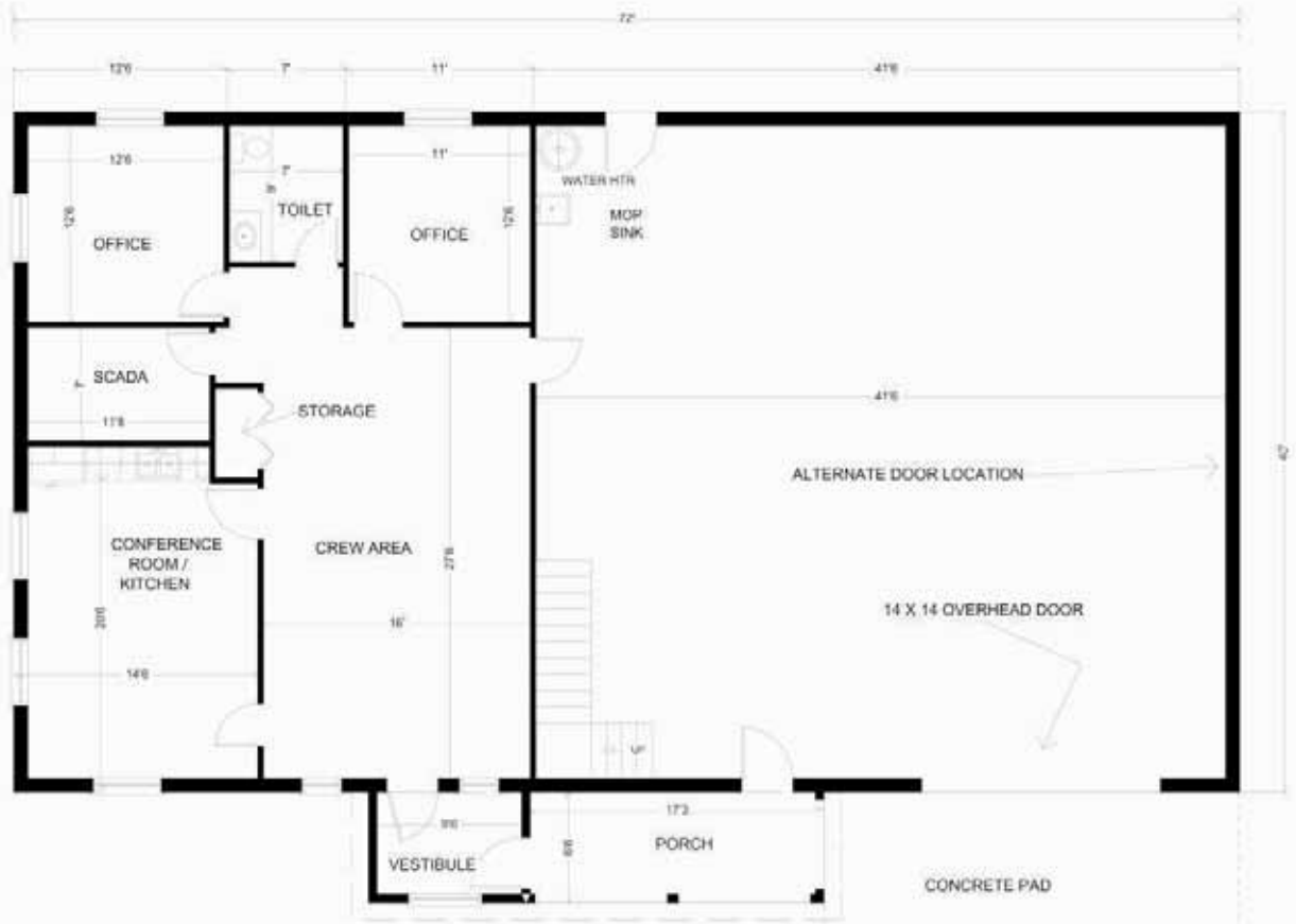
O&M BLDG FLOOR PLAN
